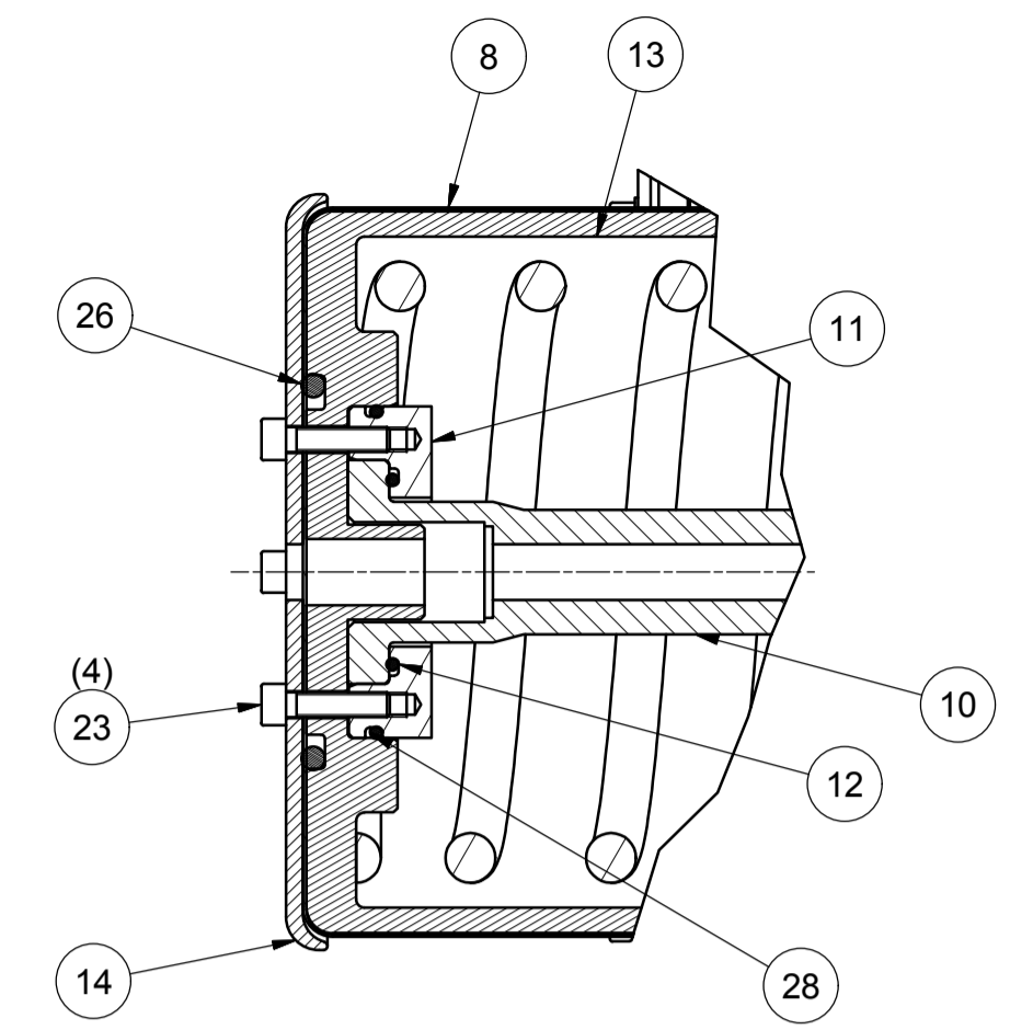
DETAIL B (1:2)
