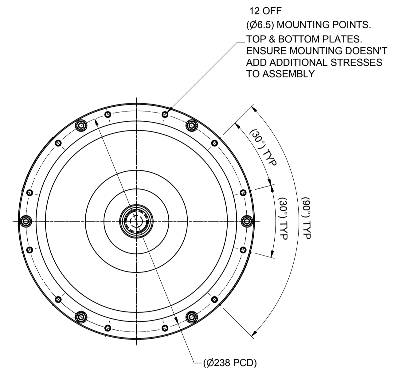
DETAIL B (1:2)
